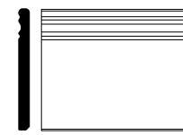
809 5.1"x6" Base Board (Glazed Top Edge)
