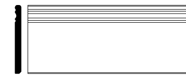
810 5.1"x12" Base Board (Glazed Top Edge)
